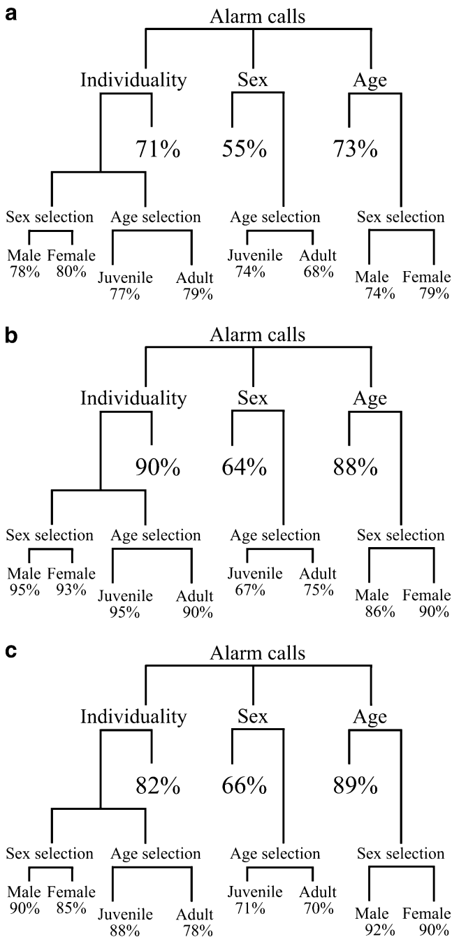
Fig. 2 Schematic representation for DFA values of correct assignment of alarm calls to individual, sex, and age: a speckled ground squirrels S. suslicus , N=96 animals; b yellow ground squirrels S. fulvus , N=100 animals; c yellow-bellied marmots M. flaviventris , N=85 animals
