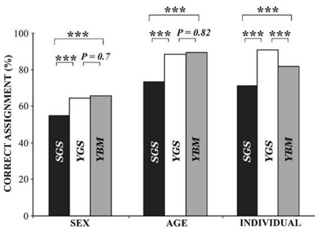
Fig. 3 Comparison between DFA values of correct assignment to sex, age, and individual for speckled ground squirrels S. suslicus (SGS), yellow ground squirrels S. fulvus (YGS), and yellow-bellied marmots M. flaviventris (YBM). ***— p < 0.001 , \chi^2 test
