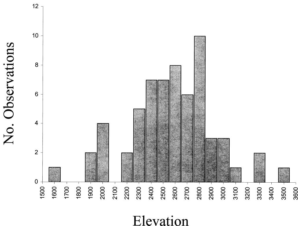
Fig. 5. Distribution of elevations (m above sea level) of 62 locations where yellow-bellied marmots ( Marmota flaviventris ) or marmot scats were found on 18 Great Basin mountain ranges during 1999–2002.
