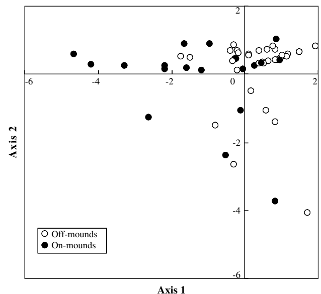
Fig. 2. Principal components analysis of the pollinator community composition for the off-mound and on-mound plots.
