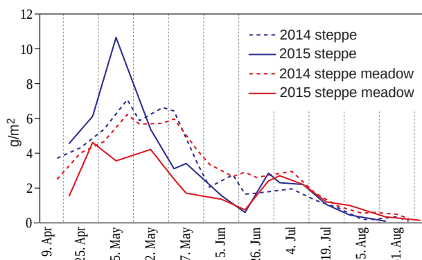
Figure 6: Daily plant regrowth during the growing seasons of 2014 and 2015 in the communities with frequently repeated mowing.
