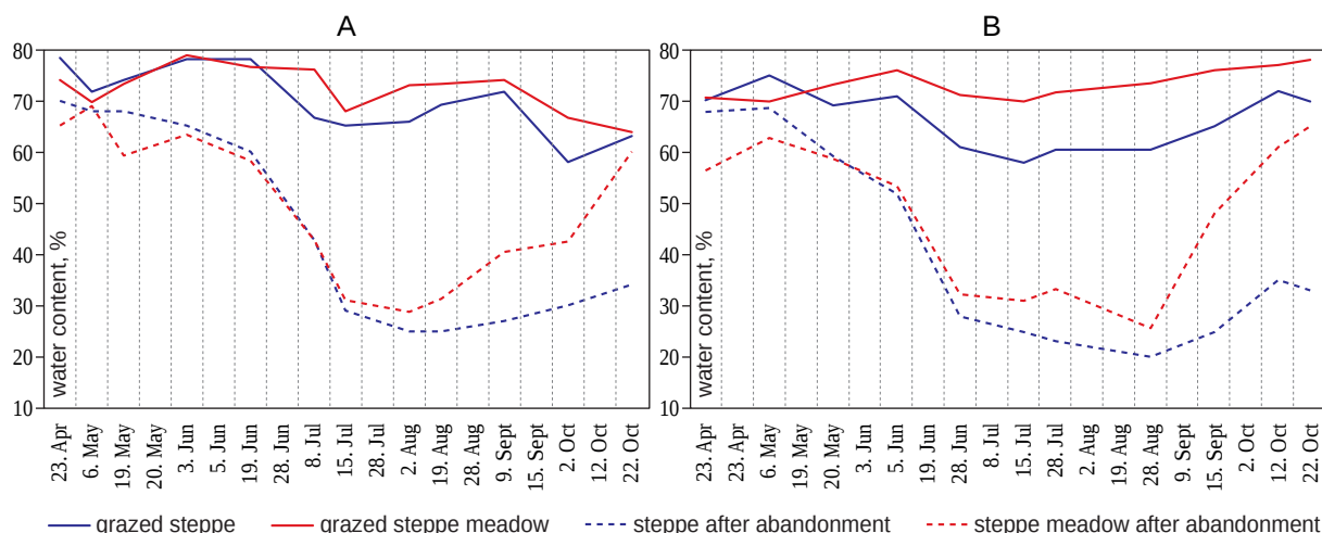
Figure 5: Water content of plant biomass during the growing seasons of 2012 (A) and 2013 (B) in the grazed and abandoned communities.
