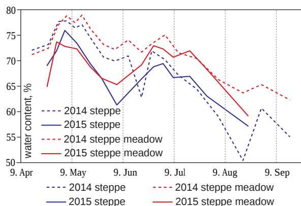
Figure 7: Water content of the plant biomass during the growing seasons of 2014 and 2015 in the communities with frequently repeated mowing.
