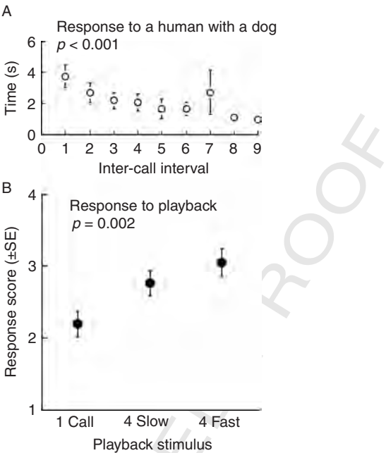
FIG. 3. (A) The response of yellow-bellied marmots to a human approaching with a dog. The intercall interval 1 = the time between the first and second call, intercall interval 2 = the time between the second and third call, and so forth. Intercall interval decreased significantly ( p < 0.01 ) demonstrating that marmots emitted calls at a faster pace as risk increased. (B) Yellow-bellied marmots responded to both the number and rate of calls played back to them. Responses were scored: 0 = no response; 1 = stand and look, 2 = rear and look, 3 = rear-up on hind legs in upright position and look, and 4 = retreat to burrow. All calls were played back at 93 dB SPL.
